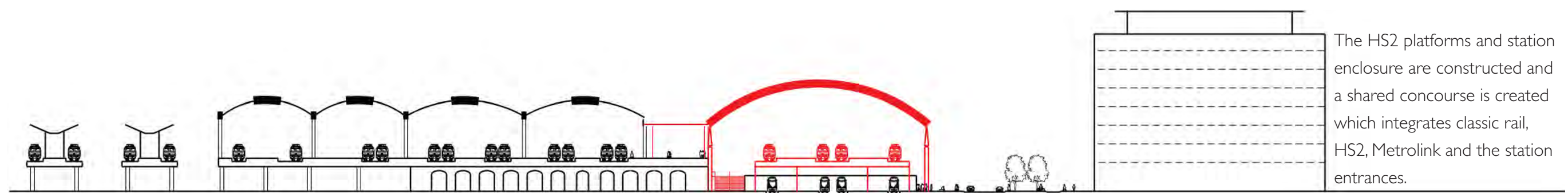
Cross Section Metrolink HS2
